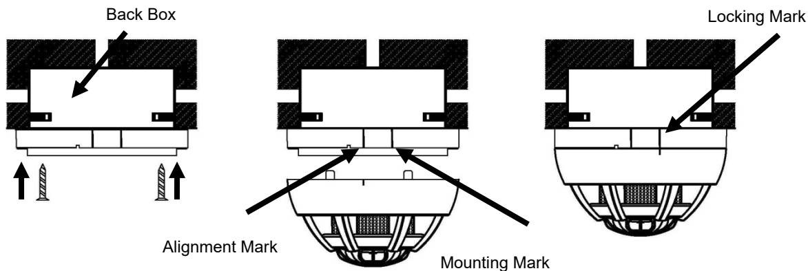
Fig.2 Mounting
